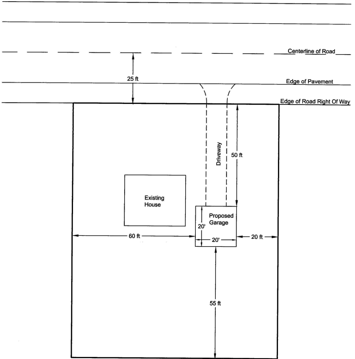
Sample Sketch Plan
